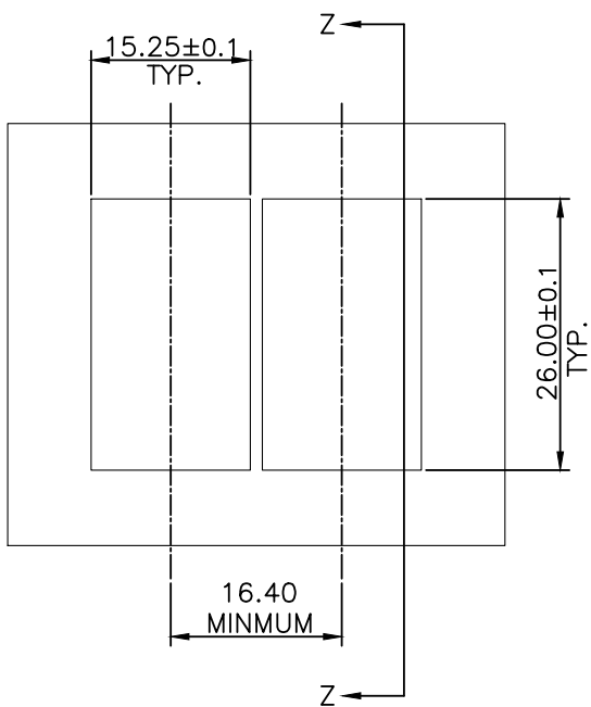
BEZEL CUT-OUT CENTER SPACING DETAIL
