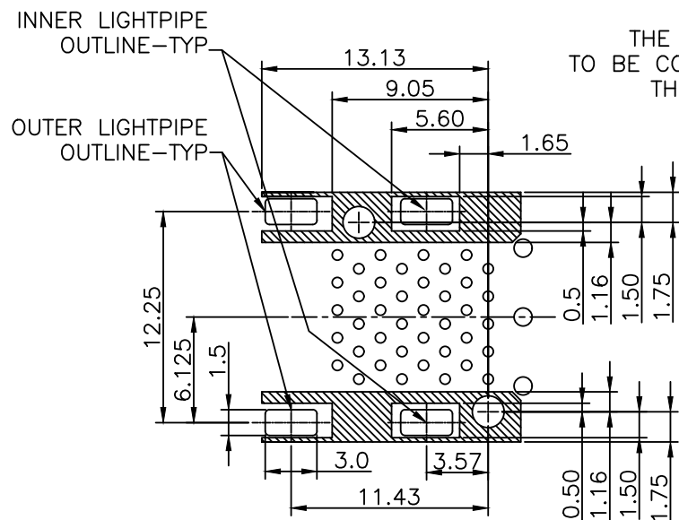
DETAIL-KEEPOUT ZONES
