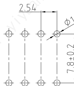
PCB LAYOUT
