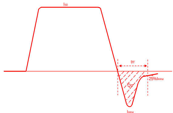
Figure D. Diode Recovery Test Circuit & Waveform
