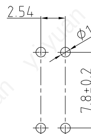
PCB LAYOUT
