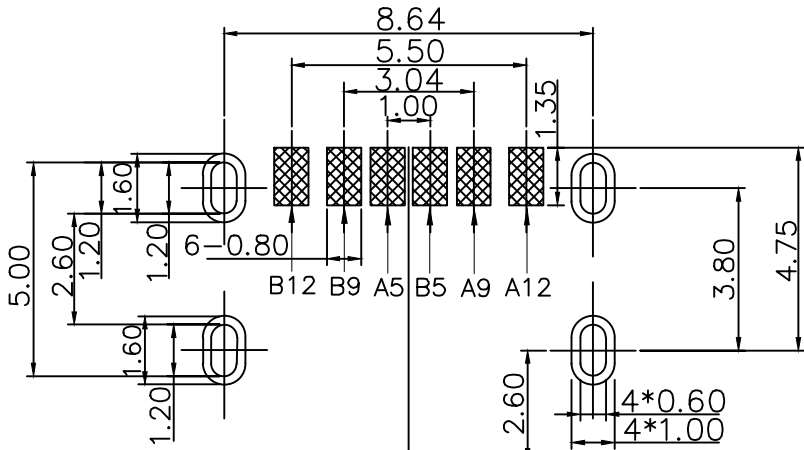
RECOMMENDED P.C.B LAYOUT TOLERANCE UNSPECIFIED ±0.05mm
