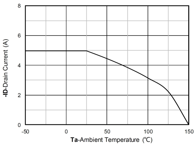
Current dissipation
