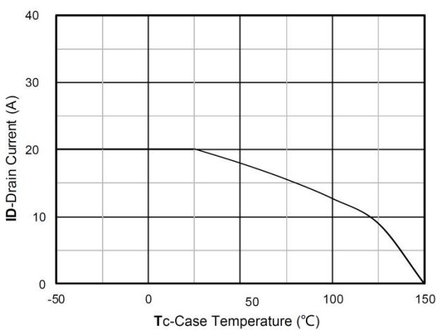
Current dissipation
