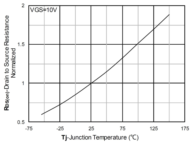
Normalized On-Resistance
