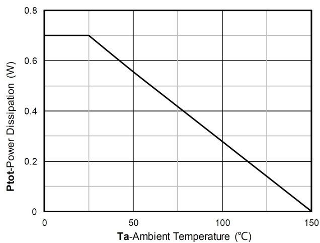
Power dissipation
