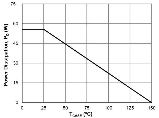
Power De-rating
