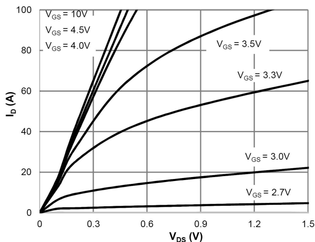
Saturation Characteristics
