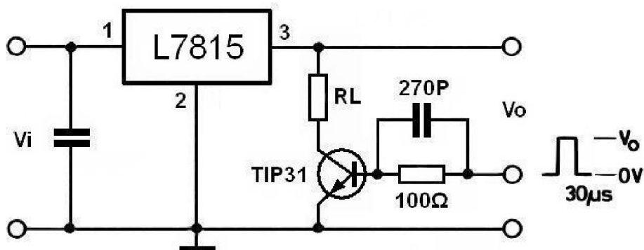
Figure 2. Load Regulation
