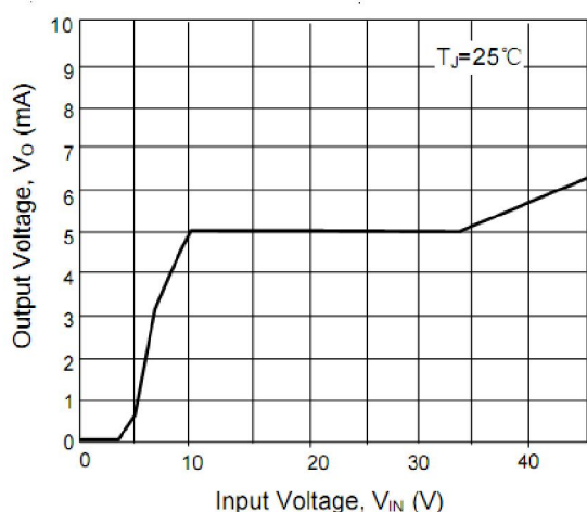
Figure 1. Output Voltage vs. Input Voltage
