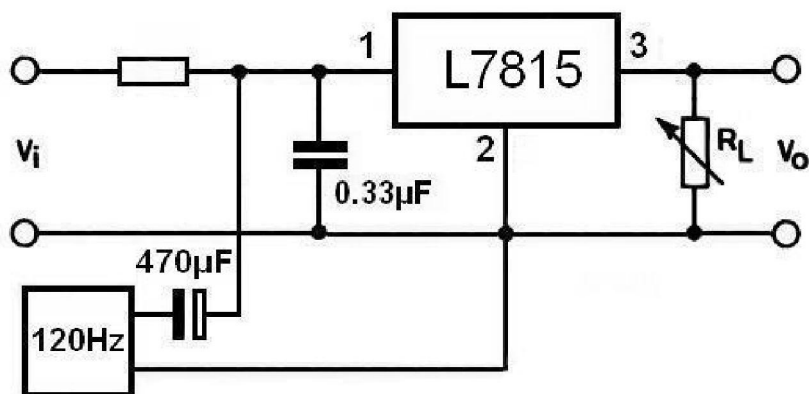
Figure 3. Ripple Rejection
