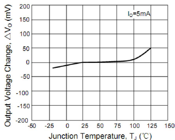
Output Voltage Change vs. Junction Temperature
