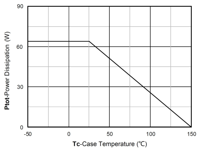
Power dissipation
