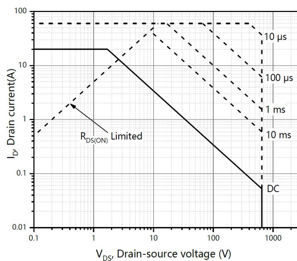
Safe operation area T_C=25^\circ C
