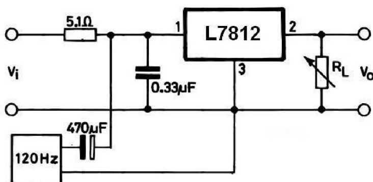
Ripple Rejection
