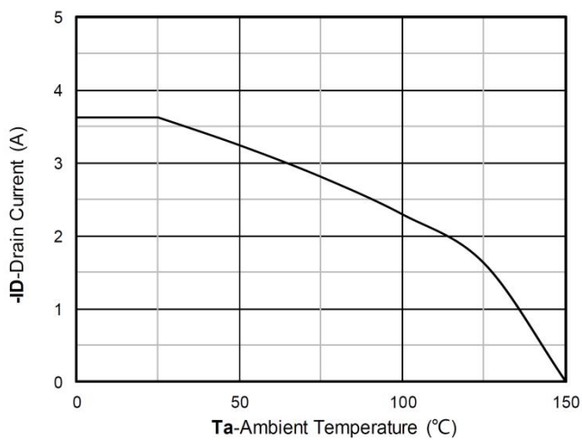
Current dissipation
