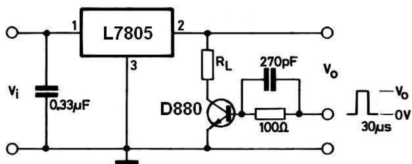
Load Regulation
