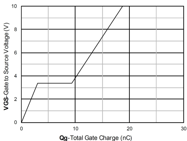
Gate Charge
