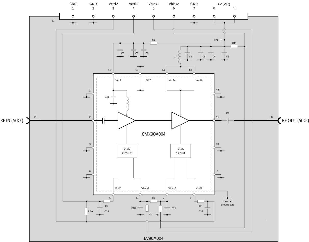
Figure 30: EV90A004 Schematic
