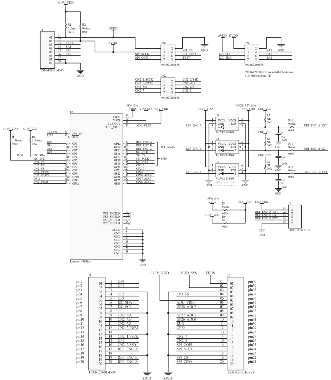
Figure 6: Schematic
