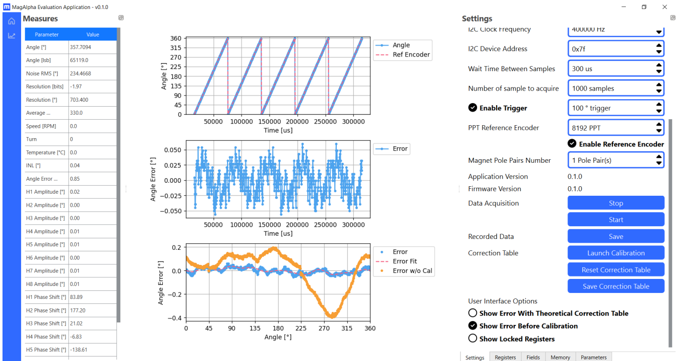
Figure 28: After MA600 Calibration
