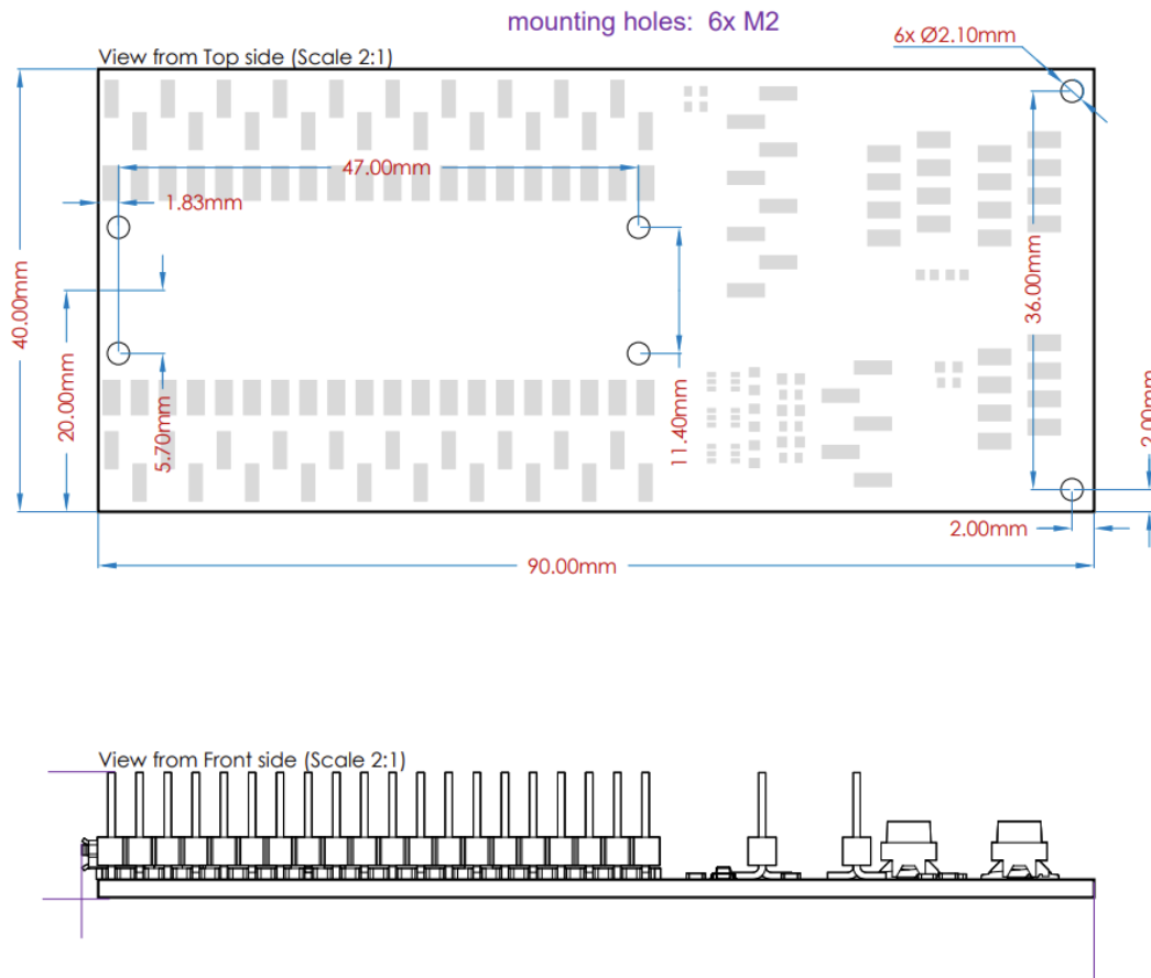
Figure 7: Mechanical Drawing
