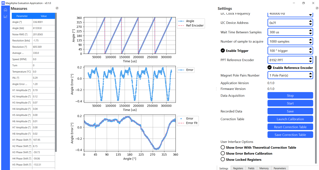
Figure 27: Before MA600 Calibration
