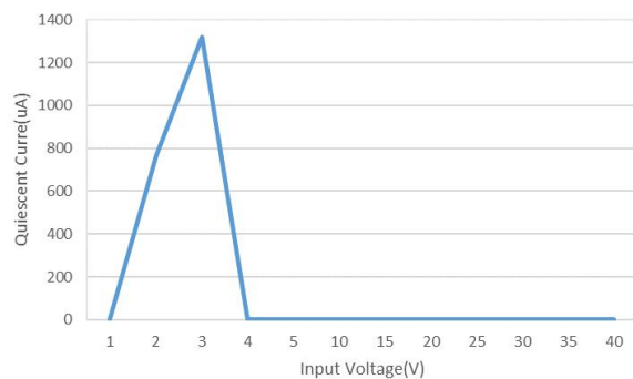
V_{IN} Vs Quiescent Current SSP7901P33PR
