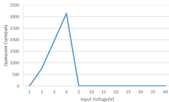
V_{IN} Vs Quiescent Current SSP7901P50PR
