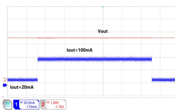
Load transient response V_{out}=3.3V , SSP7901P33PR
