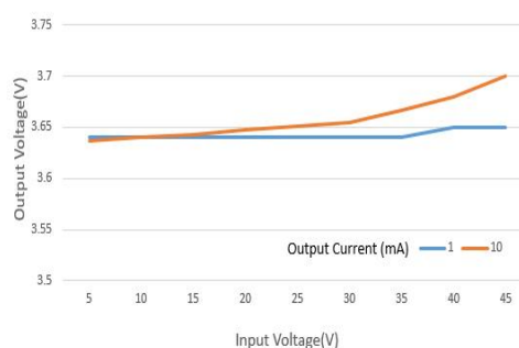
V_{OUT} vs Input Voltage SSP7903P36
