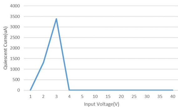
V_{IN} Vs Quiescent Current SSP7903P33
