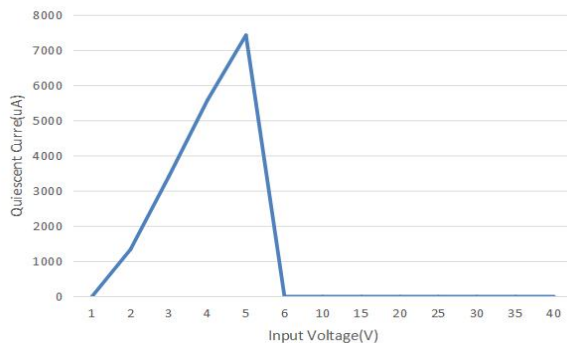
V_{IN} Vs Quiescent Current SSP7903P50
