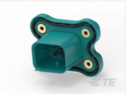
TE Part #2356408-1 4P,COAX,HDR ASSY,180DEG,COD A, SHORT
