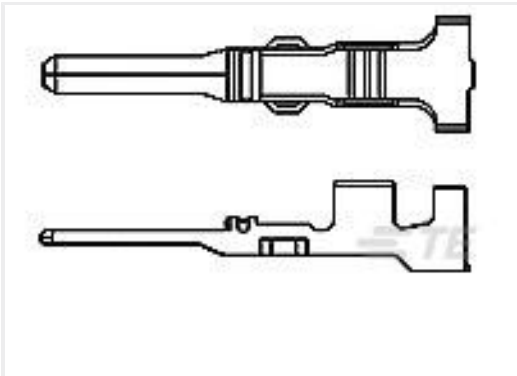
TE Part #345809-1 .070" TAB ECONOSEAL 3
