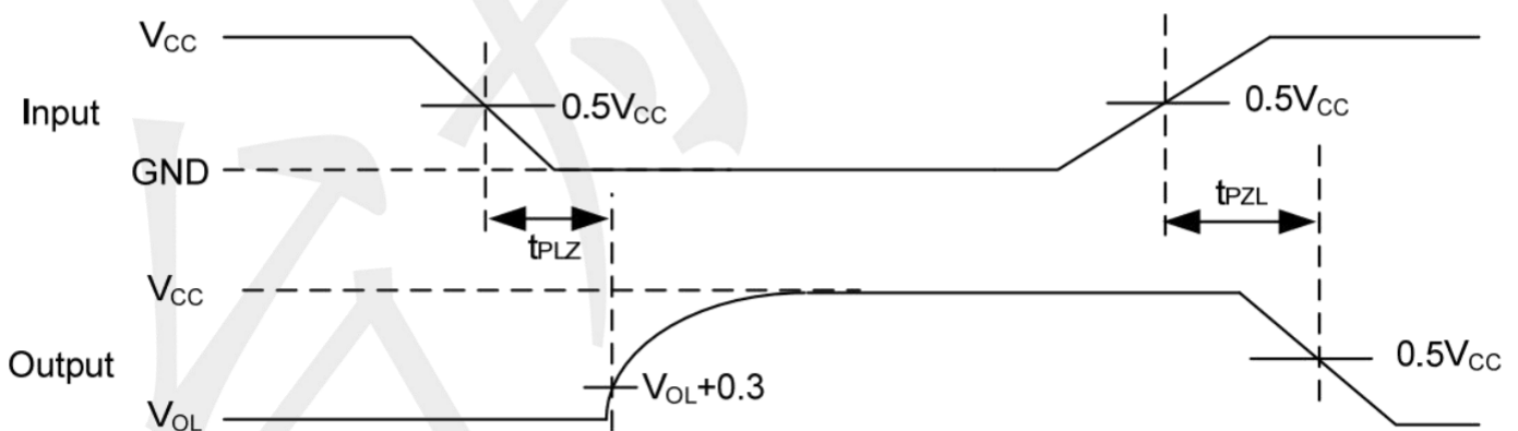
Propagation Delay Times
