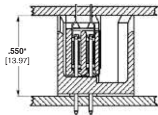
Figure 4 Double-Row, Two-Piece Receptacle and Two-Piece Shrouded Header *Mod II Shrouded Header Height is .440 [11.18] for a total stack height of .888 [22.55]
