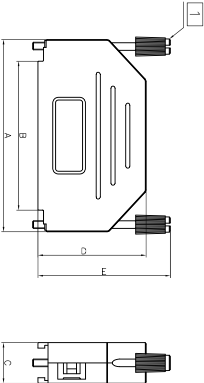
09/37 pos. Drawing for sub-assembly L17DPPK09JS/L17DPPK37JS
