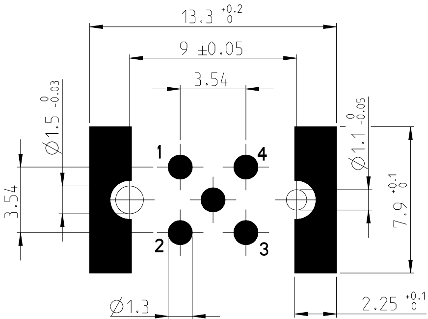
PCB-LAYOUT PROPOSAL
