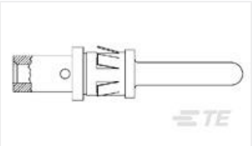
TE Part #202422-1 PIN CONT ASSY,TYPE I
