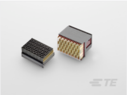
TE Part #2313237-1 RAPLUGASSY,MGRT3,POWER,DP,SE, CENTER
