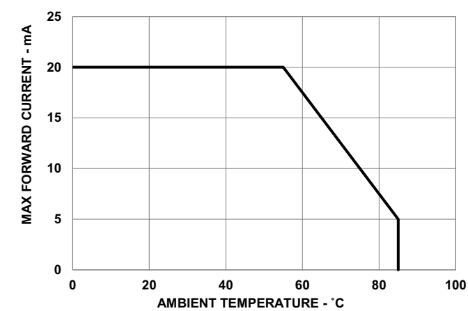
Figure 6: Derating Curve
