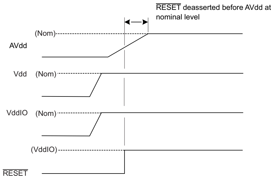
FIGURE 5-2: POWER SEQUENCING ON THE MXT449TD-AT – LATE RISE ON AVDD
