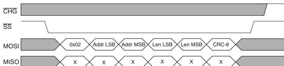
FIGURE 9-6: SPI_READ_REQ
