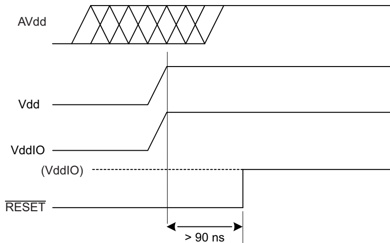
FIGURE 5-1: POWER SEQUENCING ON THE MXT449TD-AT
