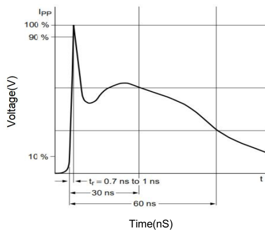
IEC61000-4-2 Pulse
