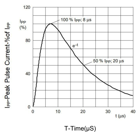
IEC61000-4-5 8X20μS Pulse
