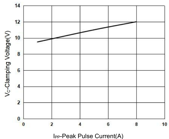
Clamping Voltage vs. Peak Pulse
