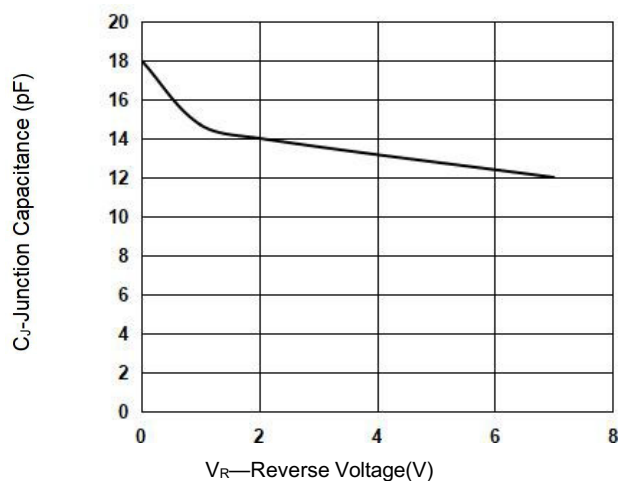
Junction Capacitance vs. Reverse
