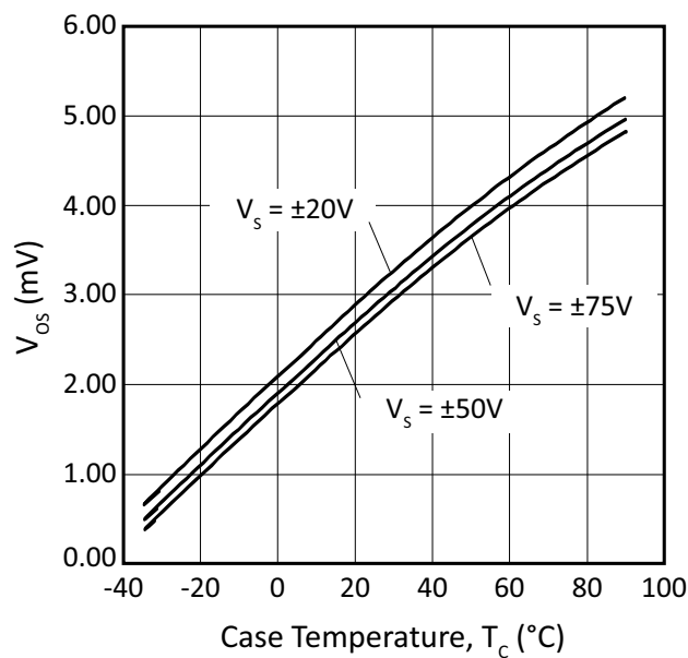
Figure 13: V OS vs. Temperature
