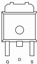
TO-252
