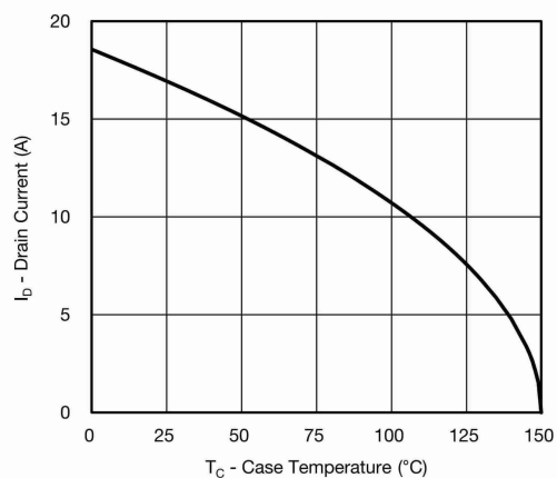
Current Derating
