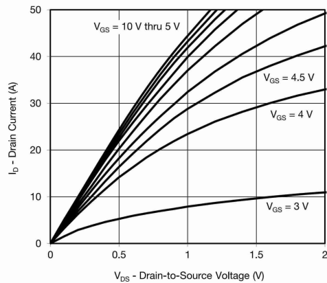
Output Characteristics
