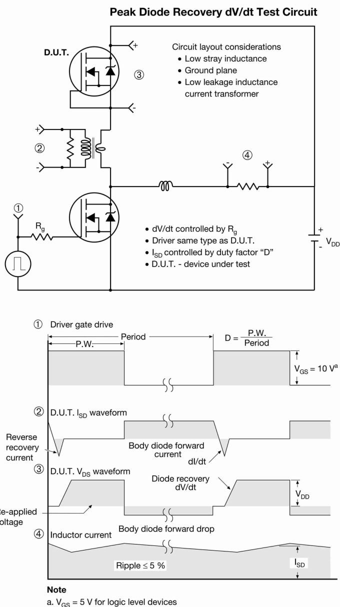
Fig. 18 - For N-Channel
