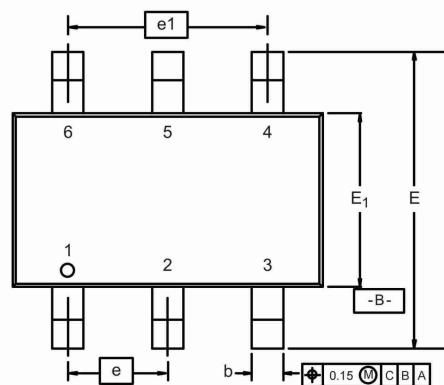
6-LEAD TSOP
