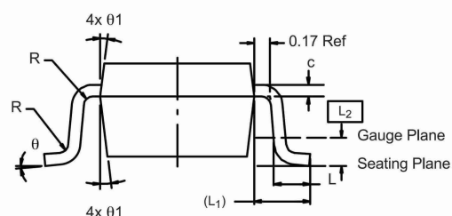
6-LEAD TSOP
