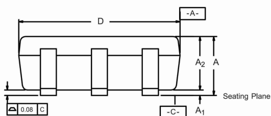
5-LEAD TSOP
