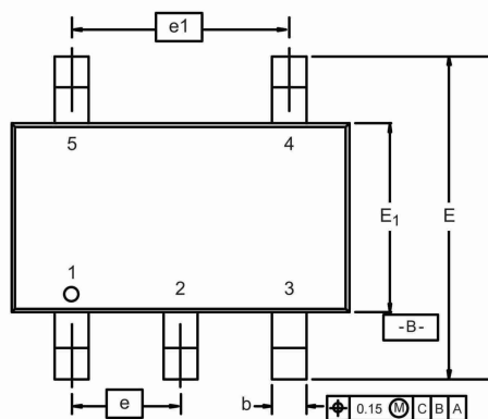
5-LEAD TSOP
