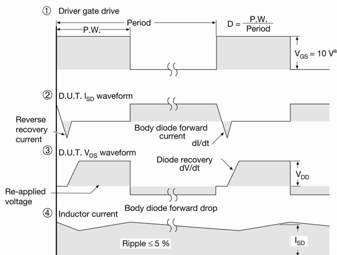
Fig. 18 - For N-Channel
