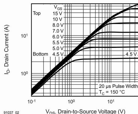
Fig. 2 - Typical Output Characteristics, T_J = 175\text{ °C}
