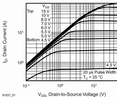
Fig. 1 - Typical Output Characteristics, T_J = 25\text{ °C}
