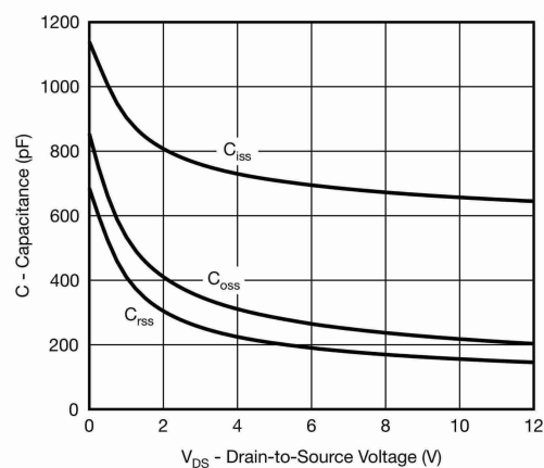
Capacitance
