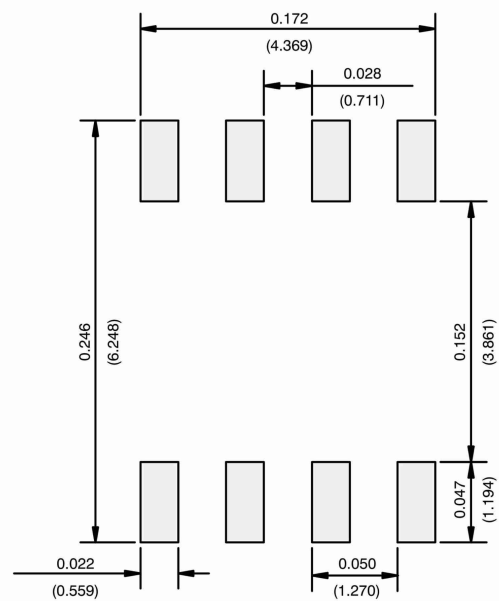
Recommended Minimum Pads Dimensions in Inches/(mm)
