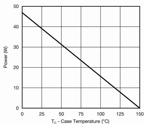
Power, Junction-to-Case
