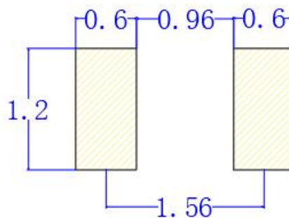
建议焊盘尺寸 Recommended Soldering Pattern
