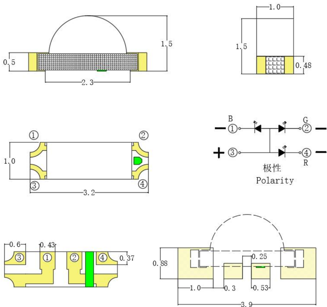
建议焊盘尺寸 Recommended Soldering Pattern
