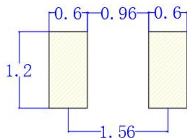
建议焊盘尺寸 Recommended Soldering Pattern
