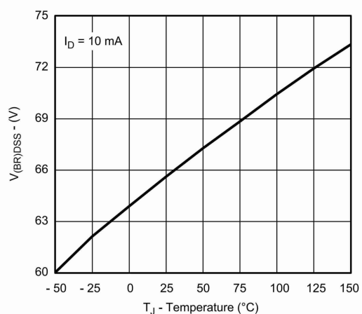
Drain-Source Breakdown Voltage vs. Junction Temperature
