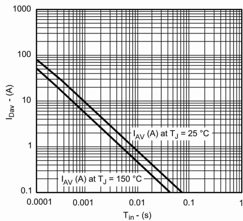
Single Pulse Avalanche Current Capability vs. Time
