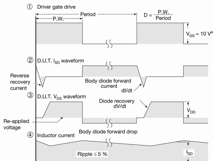
Fig. 14 - For N-Channel
