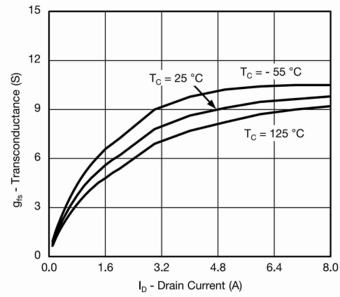
Transconductance
