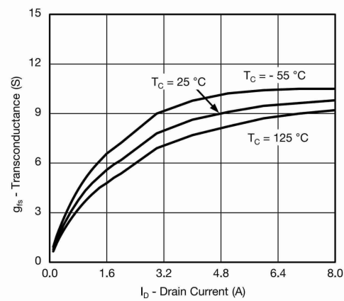
Transconductance
