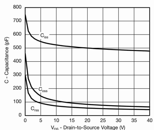
Capacitance
